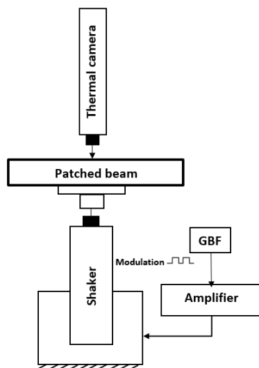
Figure 1: Experimental device
