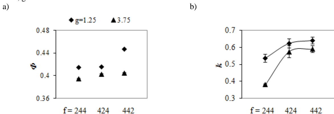
Fig. 2. Evolutions of porosity (a) and lateral-to-vertical pressure ratio (b) for mixtures with g=1.25 and g=3.75 , and different number fraction of particles.
